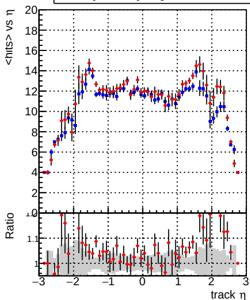
mean hits — DQM_CKF_QCDHighPt_base — DQM_mkFit_QCDHighPt_base
