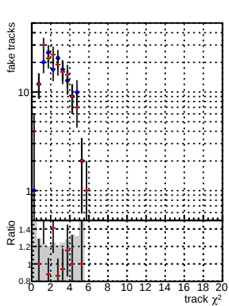
Legend: - Blue circles with error bars: DQM_CKF_QCDHighPt_base - Red circles with error bars: DQM_mkFit_QCDHighPt_base - Grey histogram: verSet
