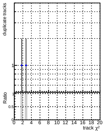
Legend: - Blue circles with error bars: DQM_CKF_QCDHighPt_base - Red circles with error bars: DQM_mkFit_QCDHighPt_base - Grey histogram: verSet
