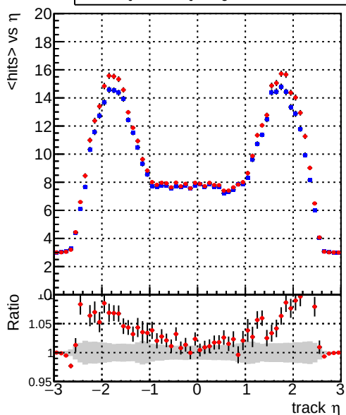
mean hit — DQM_CKF_QCDHighPt_base — DQM_mkFit_QCDHighPt_base
