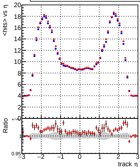
mean hit — DQM_CKF_QCDHighPt_base — DQM_mkFit_QCDHighPt_base
