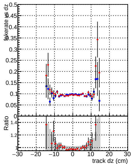
—•— DQM CKF QCDHighPt_base —•— DQM_mkFit QCDHighPt_base
