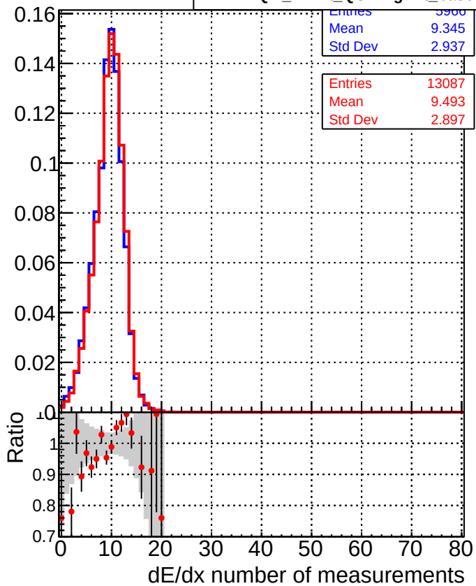
■ DQM_CKF_QCDHighPt_base ● DQM_mkFit_QCDHighPt_base
