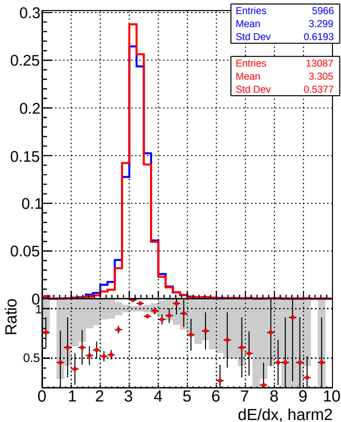
■ DQM_CKF_QCDHighPt_base ● DQM_mkFit_QCDHighPt_base
