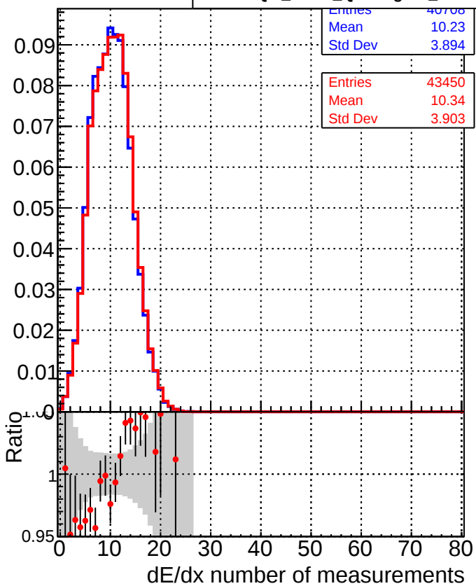
—■— DQM_CKF_QCDHighPt_base —●— DQM_mkFit_QCDHighPt_base
