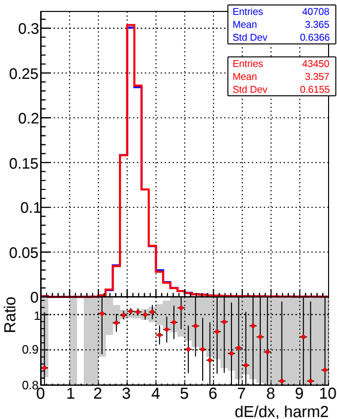
—■— DQM_CKF_QCDHighPt_base —●— DQM_mkFit_QCDHighPt_base
