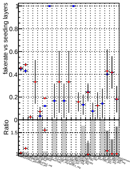
Fake rate vs. —•— DQM_CKF_QCDHighPt_base —•— DQM_mkFit_QCDHighPt_base
