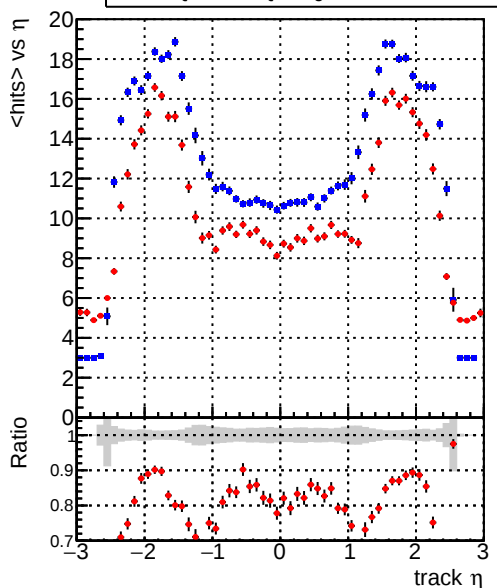
mean hits vs \eta Legend: DQM_CKF_QCDHighPt_base (blue line), DQM_mkFit_QCDHighPt_base (red line)
