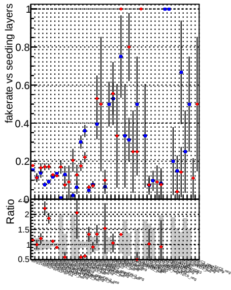
Fake rate vs. —◆— DQM_CKF_QCDHighPt_base —★— DQM_mkFit_QCDHighPt_base
