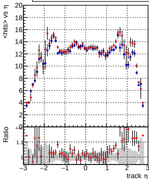
mean hits vs \eta Legend: DQM_CKF_QCDHighPt_base (blue line), DQM_mkFit_QCDHighPt_base (red line)
