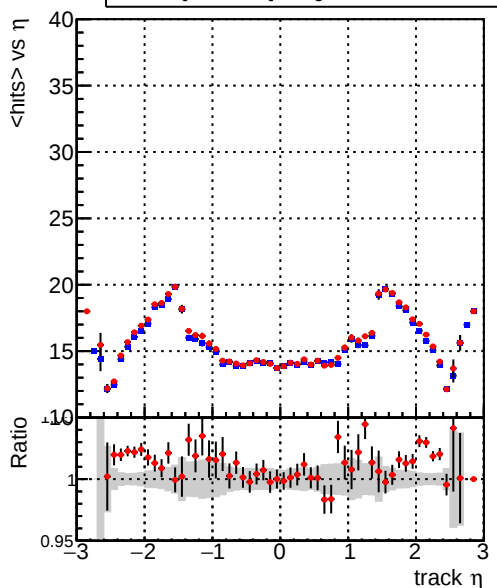
— DQM_CKF_QCDHighPt_base — DQM_mkFit_QCDHighPt_base mean hits vs \eta
