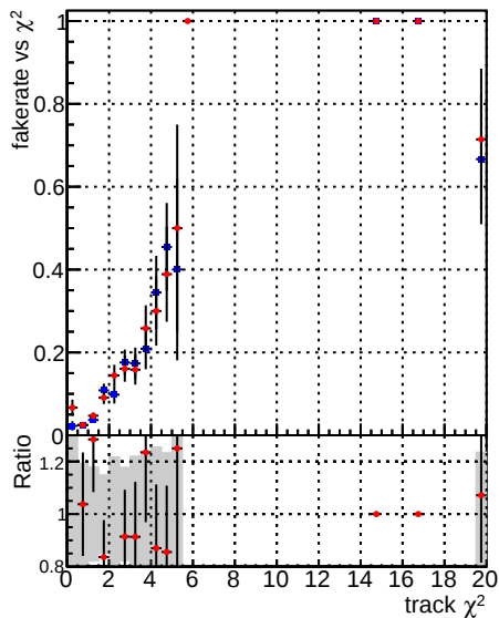
Fake rate vs. —•— DQM_CKF_QCDHighPt_base —•— DQM_mkFit_QCDHighPt_base
