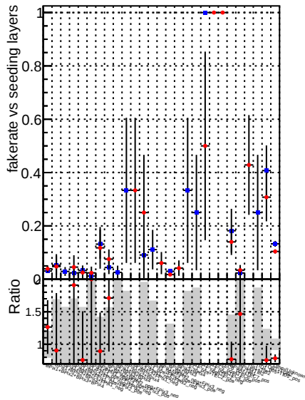
Fake rate vs. —•— DQM_CKF_QCDHighPt_base —•— DQM_mkFit_QCDHighPt_base
