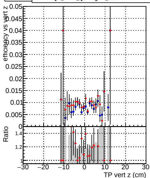
Efficiend —●— DQM_mkFit_QCDHighPt_base
