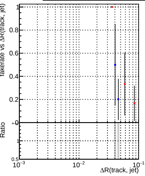
Fake rate vs \Delta R(\text{track, jet}) Legend: DQM_CKF_QCDHighPt_base (blue), DQM_mkFit_QCDHighPt_base (red)
