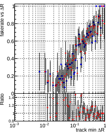
Fake rate vs \Delta R(\text{track, jet}) Legend: DQM_CKF_QCDHighPt_base (blue), DQM_mkFit_QCDHighPt_base (red)
