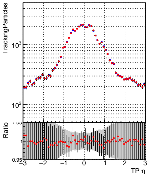
—•— DQM_CKF_QCDHighPt_base —•— DQM_mkFit_QCDHighPt_base
