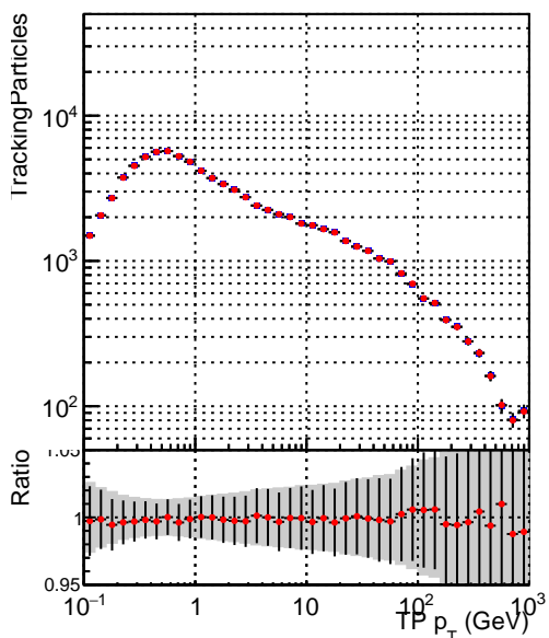
—•— DQM_CKF_QCDHighPt_base —•— DQM_mkFit_QCDHighPt_base
