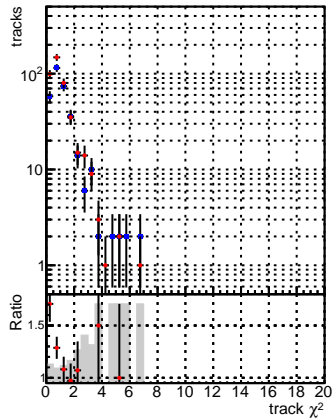
—•— DQM_CKF_QCDHighPt_base —•— DQM_mkFit_QCDHighPt_base
