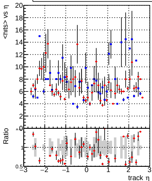
— DQM_CKF_QCDHighPt_base — DQM_mkFit_QCDHighPt_base mean hit
