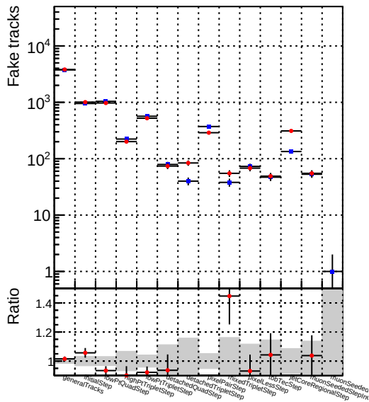
Number —●— DQM_mkFit_QCDHighPt_base
