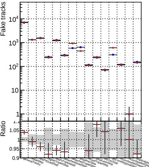
Number —●— DQM_mkFit_QCDHighPt_base
