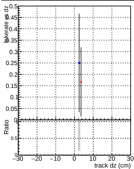
—•— DQM_CKF_QCDHighPt_base —•— DQM_mkFit_QCDHighPt_base
