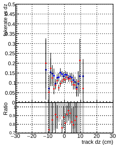
—•— DQM CKF QCDHighPt_base —•— DQM mkFit QCDHighPt_base
