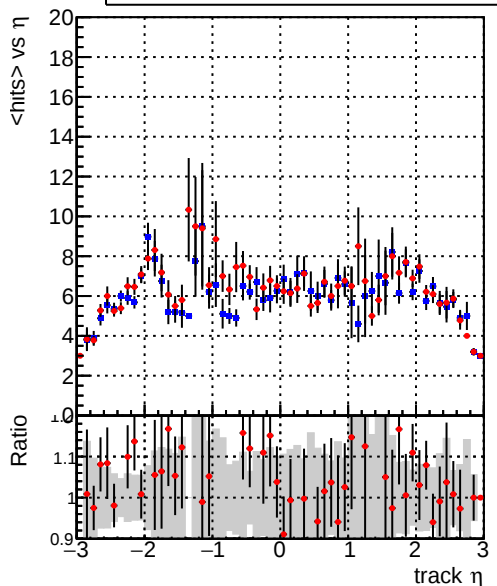
mean hits — DQM_CKF_QCDHighPt_base — DQM_mkFit_QCDHighPt_base
