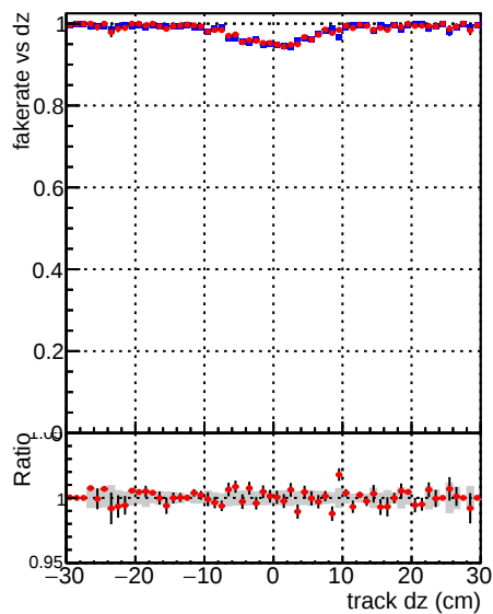
—•— DQM_CKF_QCDHighPt_base —•— DQM_mkFit_QCDHighPt_base
