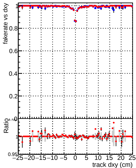
—•— DQM_CKF_QCDHighPt_base —•— DQM_mkFit_QCDHighPt_base
