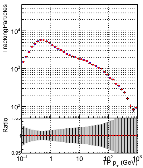
■ DQM_CKF_QCDHighPt_base ■ DQM_mkFit_QCDHighPt_base
