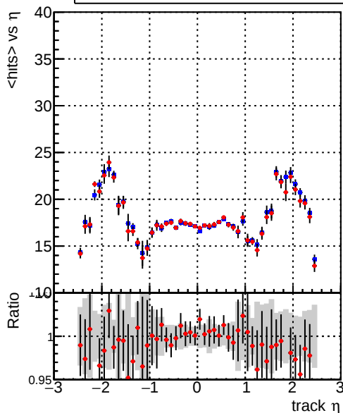
mean hits vs \eta — DQM_CKF_QCDHighPt_base — DQM_mkFit_QCDHighPt_base
