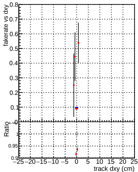
—●— DQM_CKF_QCDHighPt_base —●— DQM_mkFit_QCDHighPt_base
