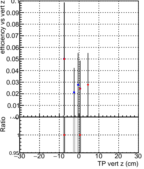
Efficiency vs vertpos —•— DQM_CKF_QCDHighPt_base —•— DQM_mkFit_QCDHighPt_base
