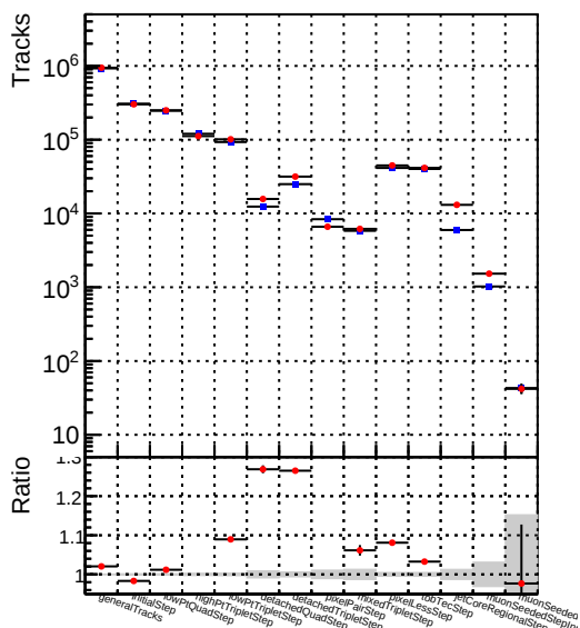
Number of tracks vs collection Legend: DQM_CKF_QCDHighPt_base (blue squares), DQM_mkFit_QCDHighPt_base (red circles)
