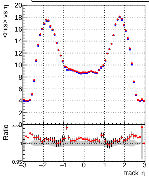
— DQM_CKF_QCDHighPt_base — DQM_mkFit_QCDHighPt_base mean hits
