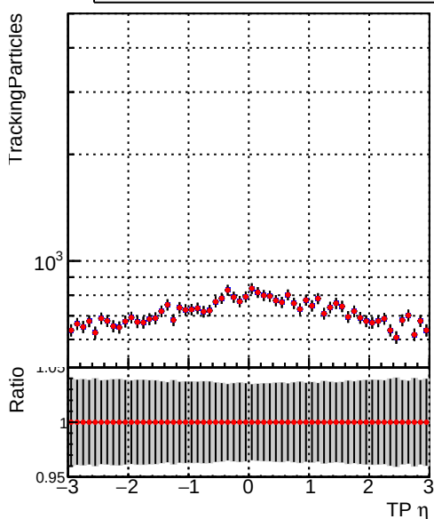
—•— DQM_mkFit_QCDHighPt_base —•— DQM_mkFit_QCDHighPt_retrain
