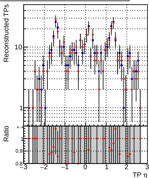
—•— DQM_mkFit_QCDHighPt_base —•— DQM_mkFit_QCDHighPt_retrain
