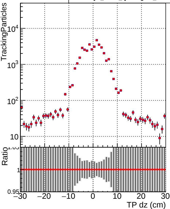
■ DQM_mkFit_QCDHighPt_base ■ DQM_mkFit_QCDHighPt_retrain
