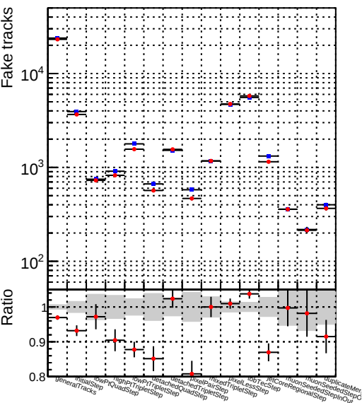
Number —●— DQM_mkFit_QCDHighPt_retrain
