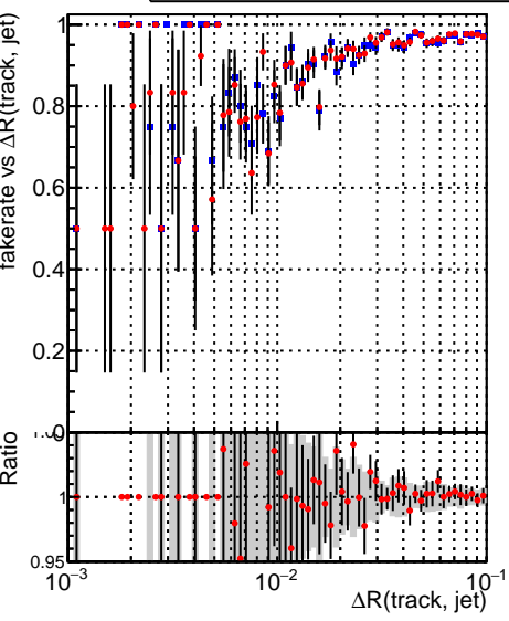
—●— DQM_mkFit_QCDHighPt_base —●— DQM_mkFit_QCDHighPt_retrain
