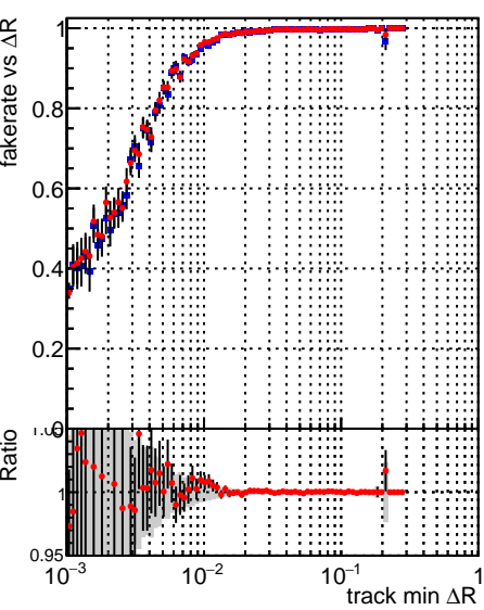
—●— DQM_mkFit_QCDHighPt_base —●— DQM_mkFit_QCDHighPt_retrain
