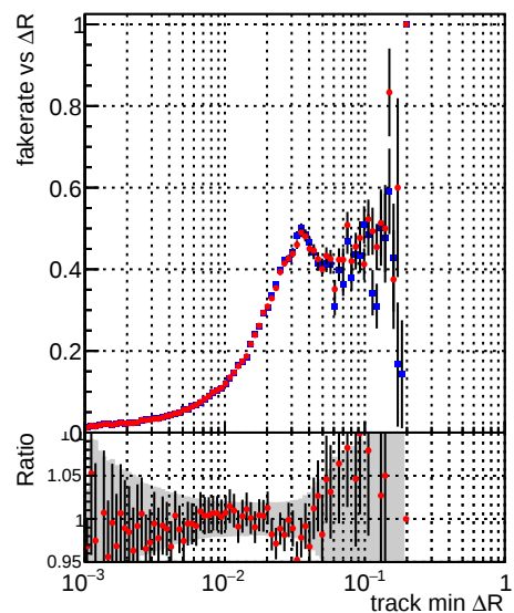
Fake rate vs —■— DQM_mkFit_QCDHighPt_base —●— DQM_mkFit_QCDHighPt_retrain
