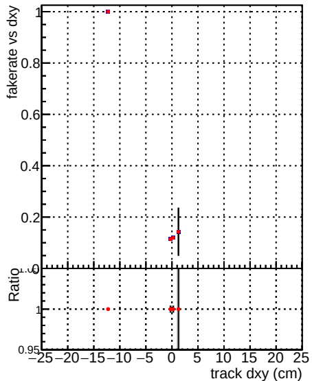
—•— DQM_mkFit_QCDHighPt_base —•— DQM_mkFit_QCDHighPt_retrain
