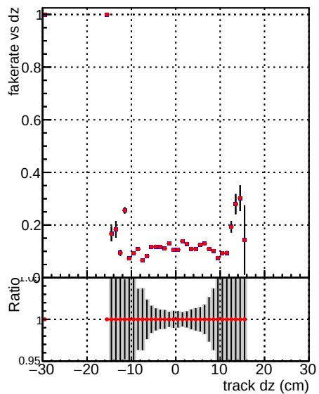
—•— DQM_mkFit_QCDHighPt_base —•— DQM_mkFit_QCDHighPt_retrain
