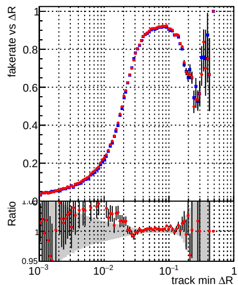
■ DQM_mkFit_QCDHighPt_base ● DQM_mkFit_QCDHighPt_retrain
