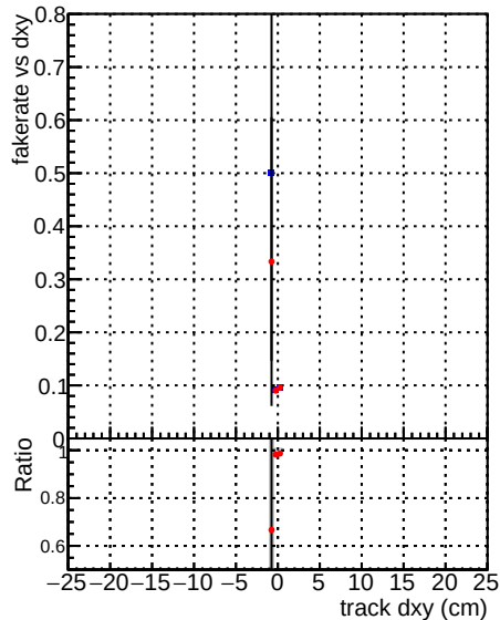
—•— DQM_mkFit_QCDHighPt_base —•— DQM_mkFit_QCDHighPt_retrain
