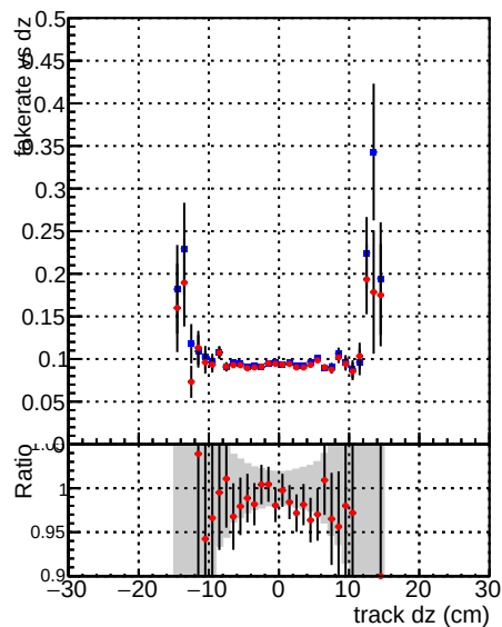
—•— DQM_mkFit_QCDHighPt_base —•— DQM_mkFit_QCDHighPt_retrain
