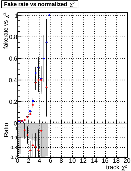
Fake rate vs. —•— DQM_mkFit_QCDHighPt_base —•— DQM_mkFit_QCDHighPt_retrain
