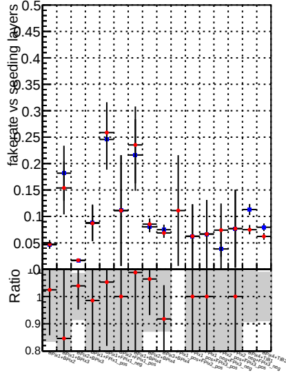
Fake rate vs. —•— DQM_mkFit_QCDHighPt_base —•— DQM_mkFit_QCDHighPt_retrain
