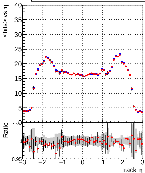
DQM_mkFit_QCDHighPt_base mean hits DQM_mkFit_QCDHighPt_retrain
