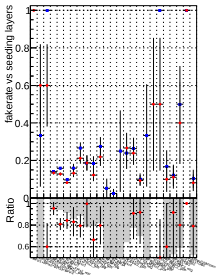
Fake rate vs. —•— DQM_mkFit_QCDHighPt_base —•— DQM_mkFit_QCDHighPt_retrain
