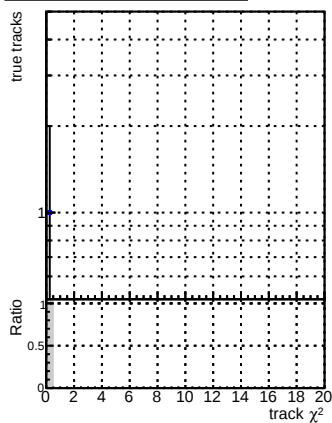
N of associated tracks vs. \chi^2
