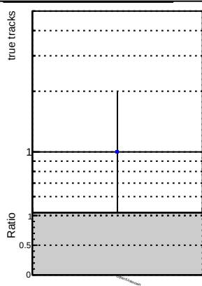
N of associated tracks vs. \chi^2
