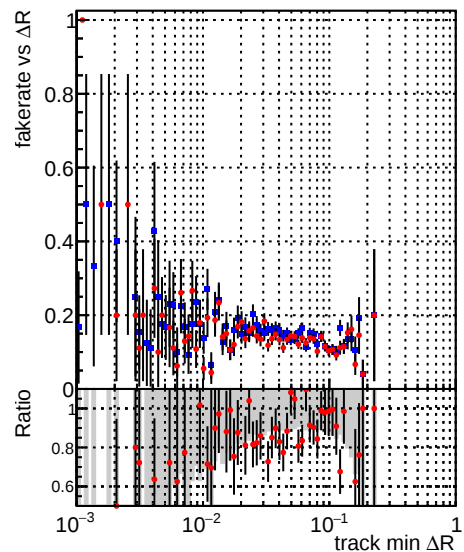
DQM_mkFit_QCDHighPt_base Fake rate vs \Delta R(\text{track, jet}) DQM_mkFit_QCDHighPt_retrain
