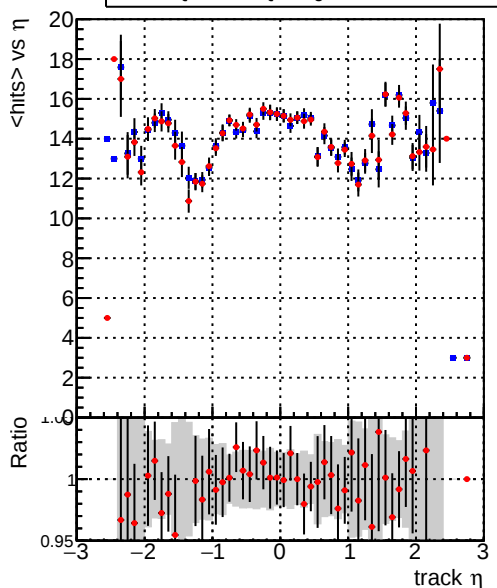
— DQM_mkFit_QCDHighPt_base — DQM_mkFit_QCDHighPt_retrain mean hits
