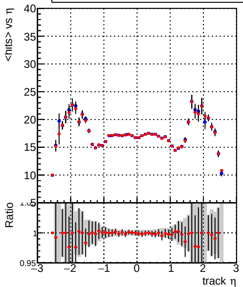
mean hit — DQM_mkFit_QCDHighPt_base — DQM_mkFit_QCDHighPt_retrain
