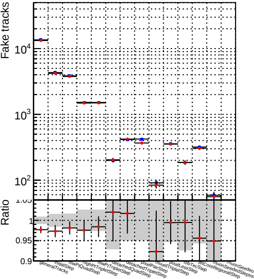
Number —●— DQM_mkFit_QCDHighPt_retrain
