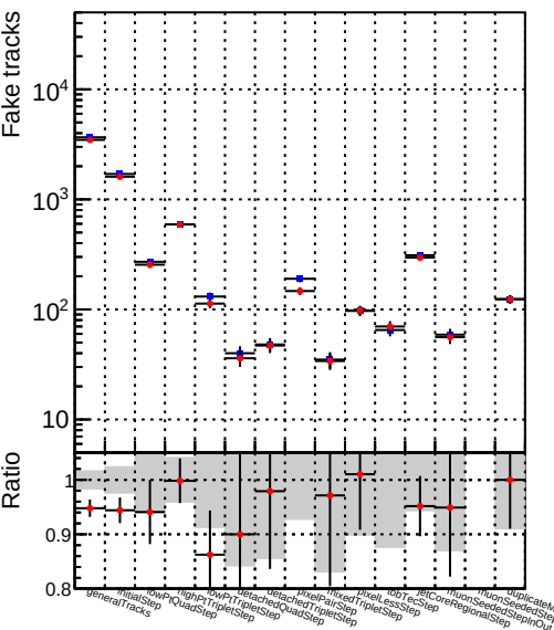
Number —●— DQM_mkFit_QCDHighPt_retrain
