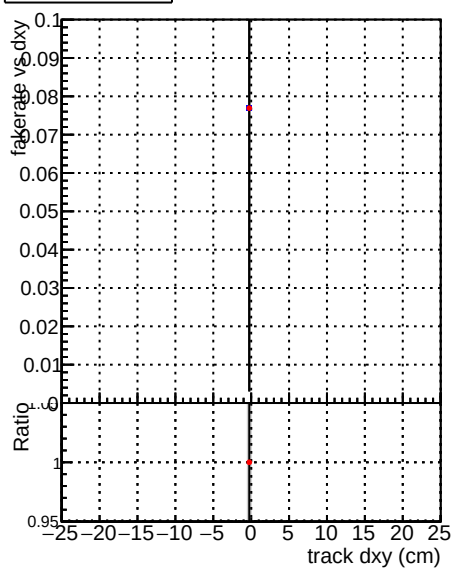
—•— DQM_mkFit_QCDHighPt_base —•— DQM_mkFit_QCDHighPt_retrain
