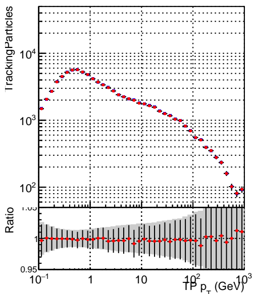
—•— DQM_mkFit_QCDHighPt_base —•— DQM_mkFit_QCDHighPt_retrain
