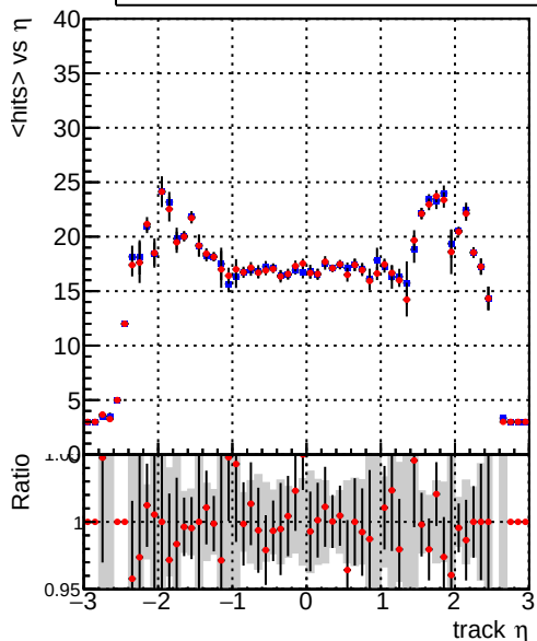
mean hits — DQM_mkFit_QCDHighPt_base — DQM_mkFit_QCDHighPt_retrain
